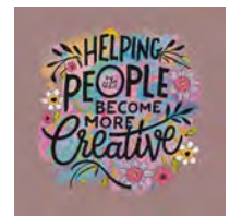
Ideogram v0.1
