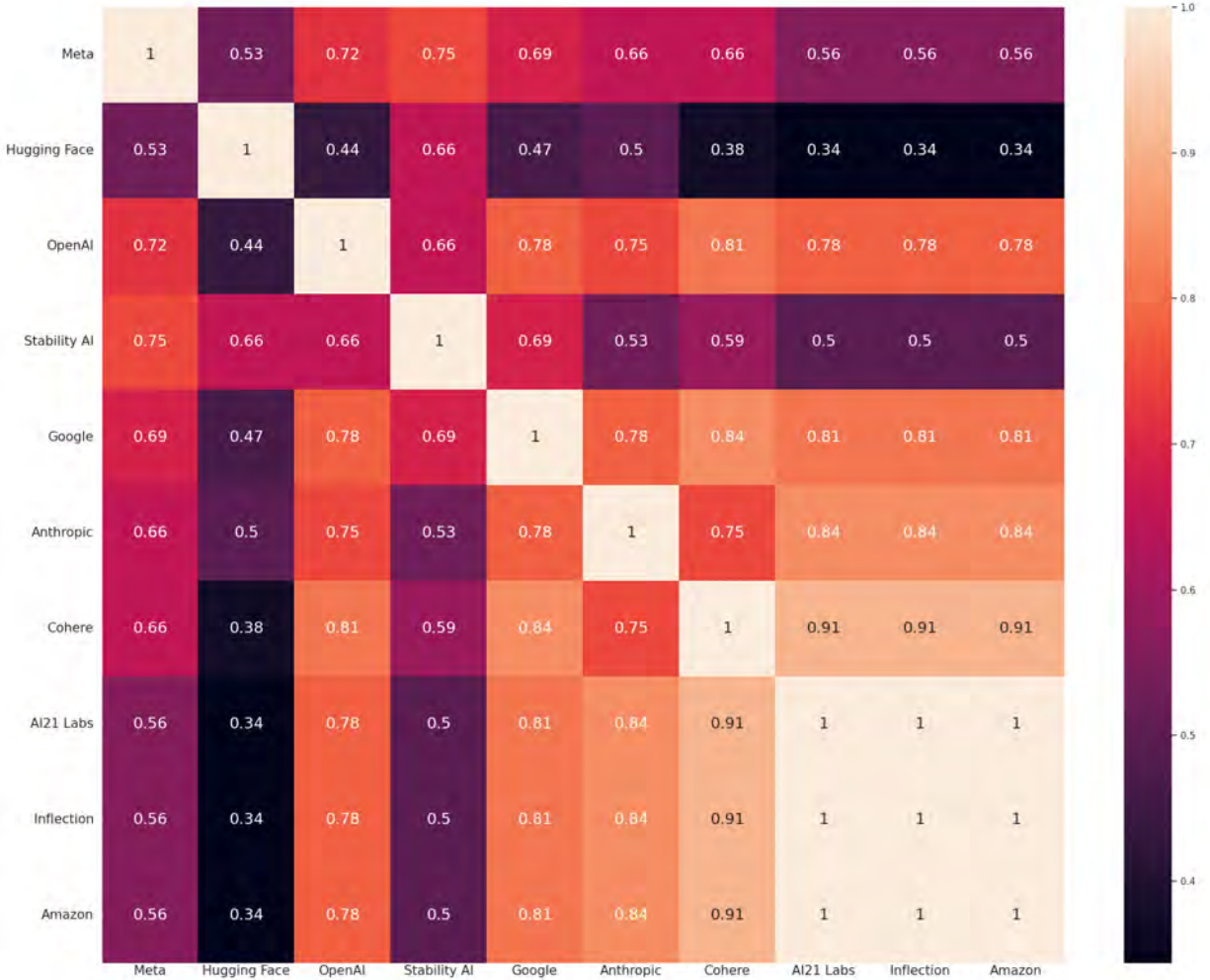
Fig. 15. Correlations between Companies (Upstream Indicators). The correlation between the scores for pairs of companies across all indicators when only considering upstream indicators. Correlation is measured using the simple matching coefficient (i.e. agreement rate), which is the fraction of all indicators for which both companies receive the same score (i.e. both receive the point or both do not receive the point).
