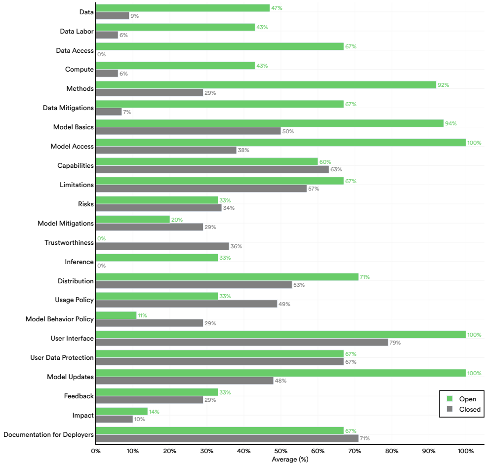
Fig. 13. Open vs. Closed by Subdomains. The mean score for the 3 open developers (Meta, Hugging Face, Stability AI) and the 7 closed developers (OpenAI, Anthropic, Google, Cohere, AI21 Labs, Inflection, Amazon) across each of the 23 subdomains. Note: the number of indicators per subdomain varies widely.
