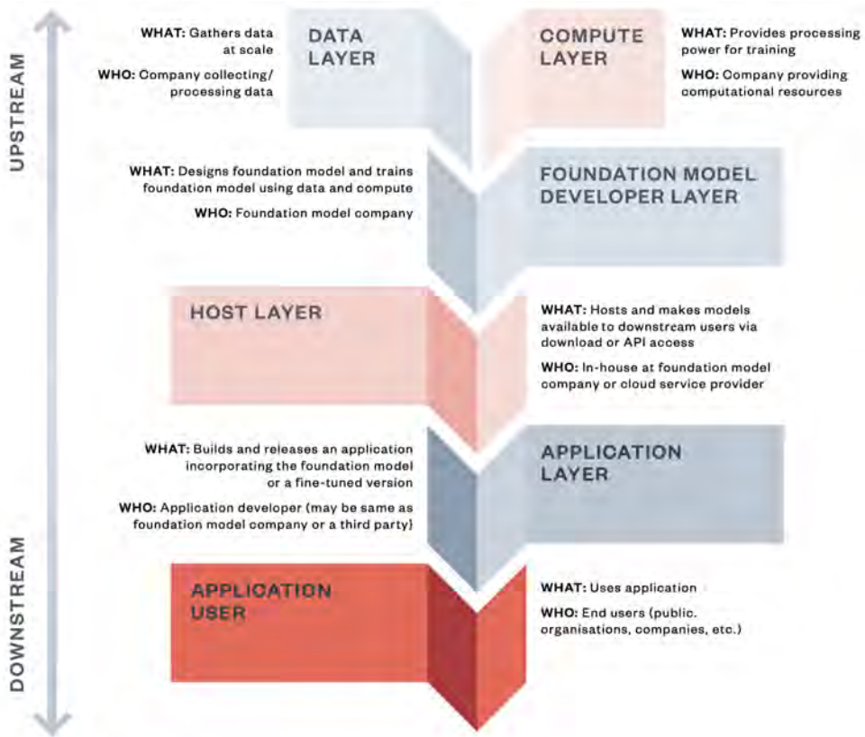
Fig. 1. Foundation Model Supply Chain. A conceptual depiction of the foundation model supply chain, beginning with the primary upstream resources (i.e. data, compute) and transitioning to the foundation model, subsequent hosts (or distribution channels ), and ending with downstream applications. Image taken with permission from Jones (2023).
