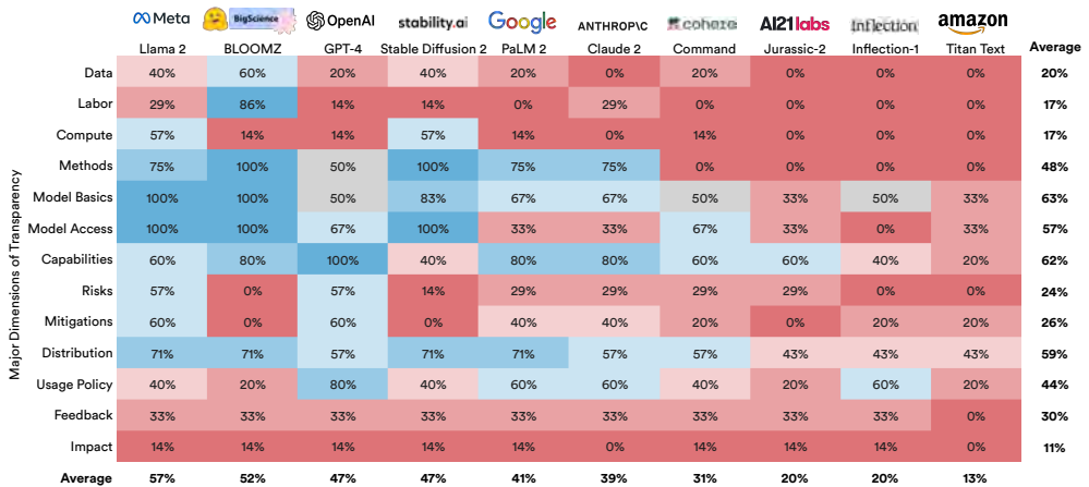
Fig. 9. Scores by Major Dimensions of Transparency. The fraction of achieved indicators in each of the 13 major dimension of transparency. Major dimension of transparency are large subdomains within the 23 subdomains.
