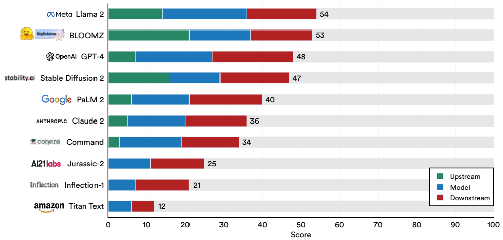
Fig. 8. Scores by Domain. The aggregate score of each developer broken down by the three domains: upstream, model, and downstream.
