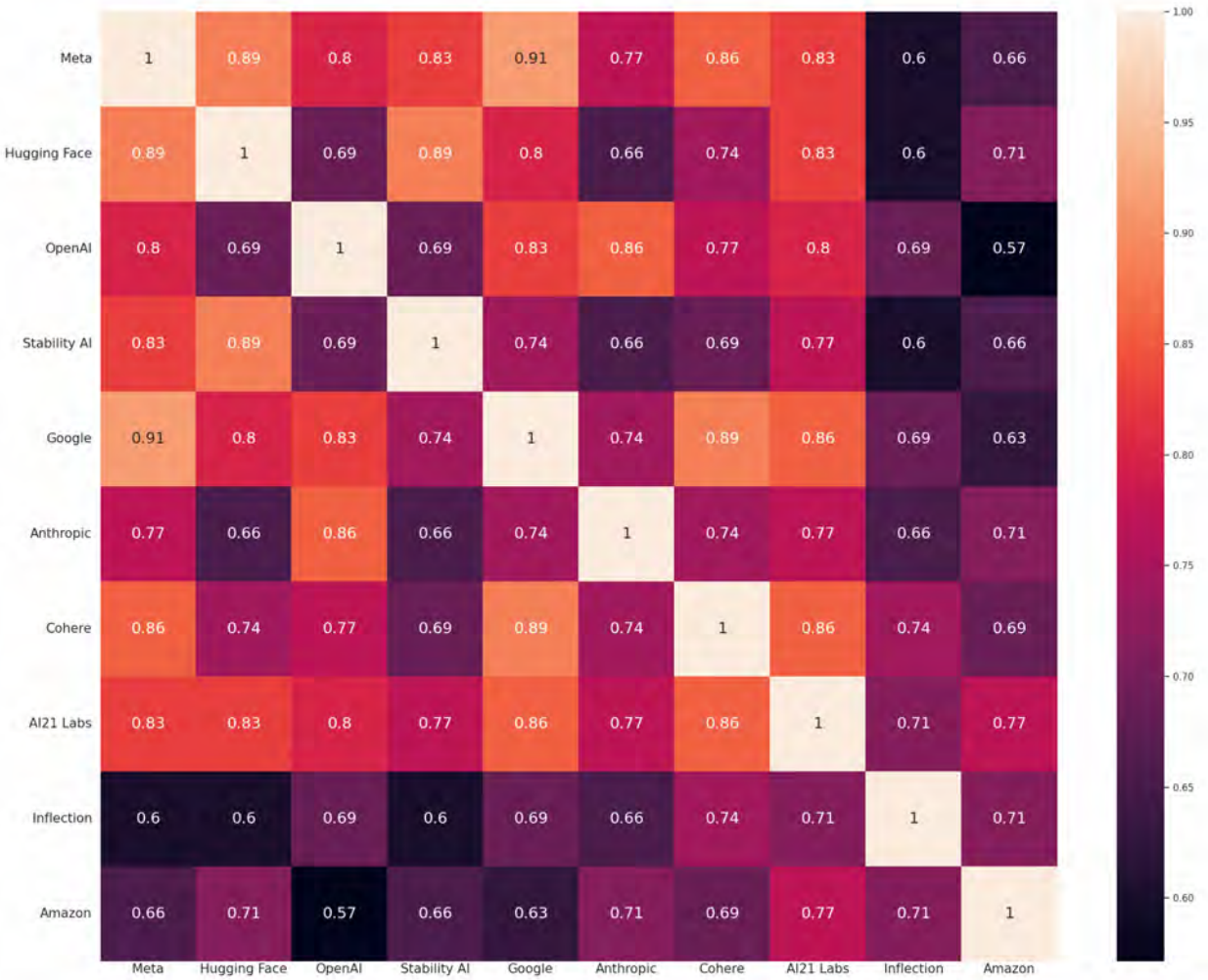
Fig. 17. Correlations between Companies (Downstream Indicators). The correlation between the scores for pairs of companies across all indicators when considering only downstream indicators. Correlation is measured using the simple matching coefficient (i.e. agreement rate), which is the fraction of all indicators for which both companies receive the same score (i.e. both receive the point or both do not receive the point).
